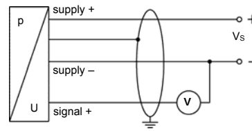
3-wire-system (voltage)
